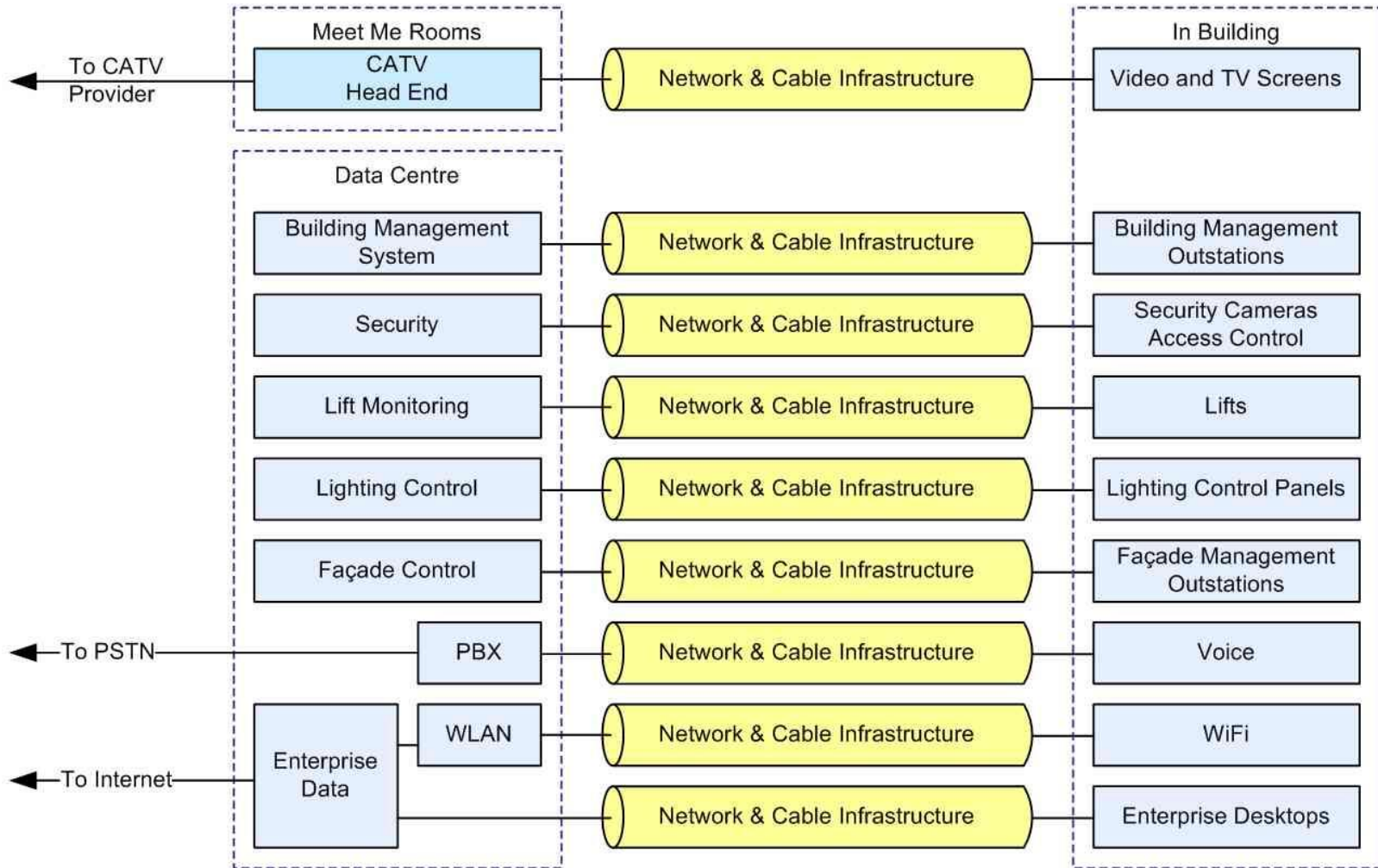
Typical In-Building Segregated Network Infrastructure
