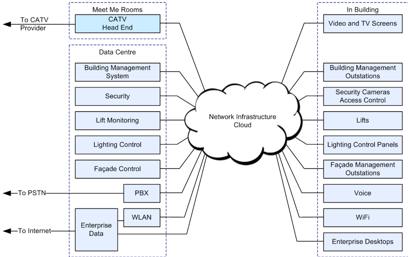
In-Building Network Infrastructure Cloud
